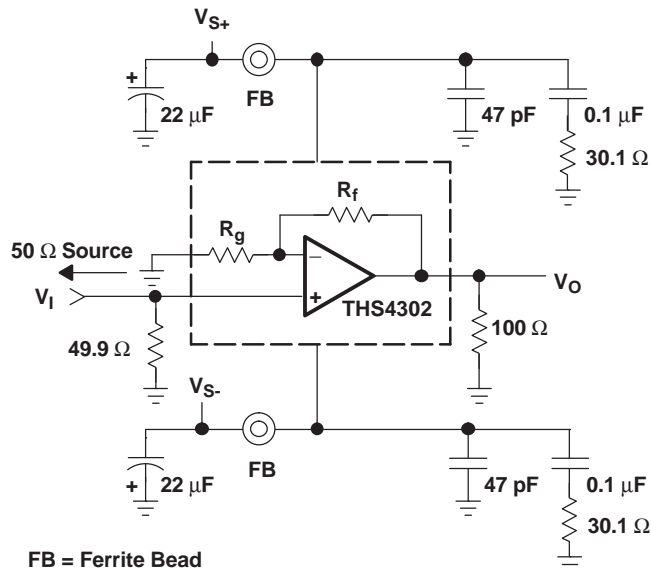
APPLICATION CIRCUIT
